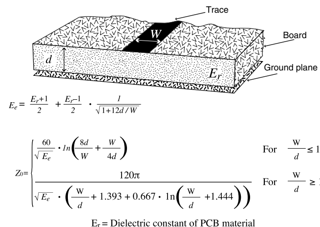
Figure 38: Microstrip Formulas
